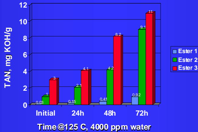
Figure 3. Residual acid left after manufacturing shortens ester life dramatically.
